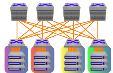
Arista Leaf-Spine Two-tier Network Architecture with 7060X and 7260X Series
