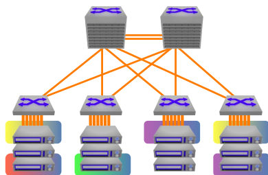
Arista Leaf-Spine Two-tier Network Architecture with 7060X and 7260X Series
