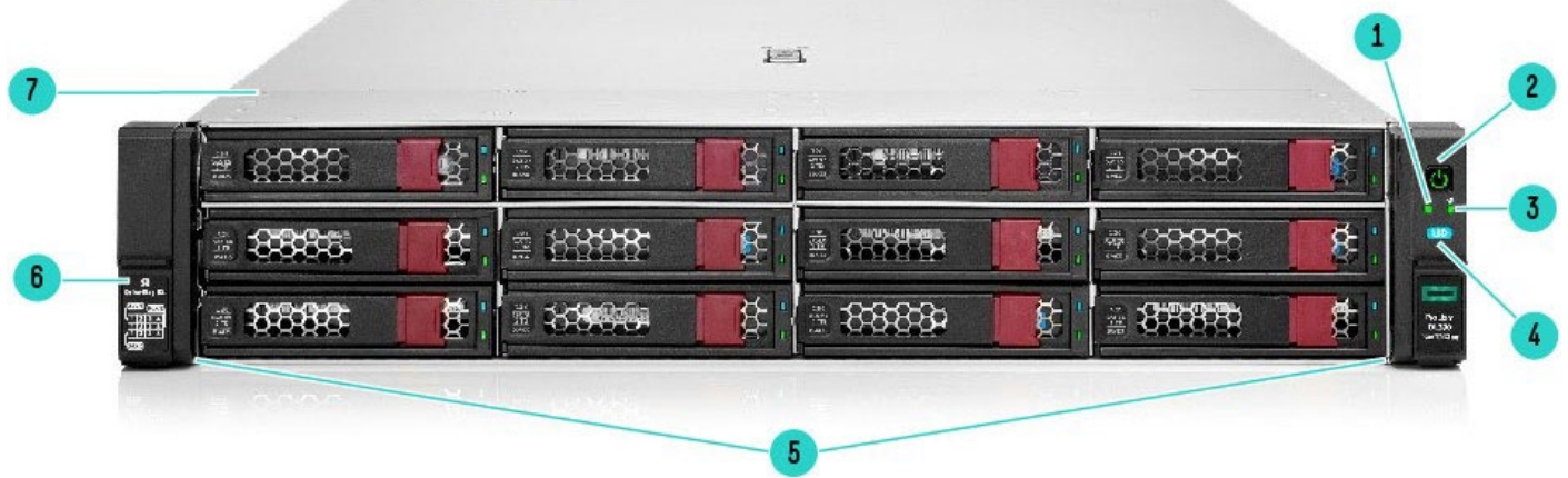
Front View – 12LFF chassis shown
