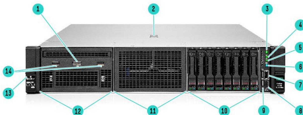
Front View – SFF chassis with optional Universal Media Bay shown
